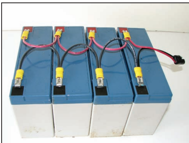
Battery Wired for 6 volts
